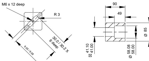
Vane Slot detail both ends
